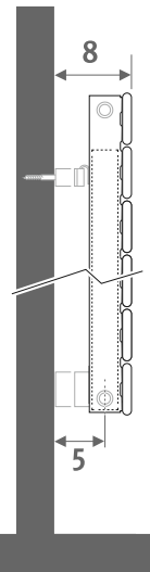
Type 11 extended wall fixing
