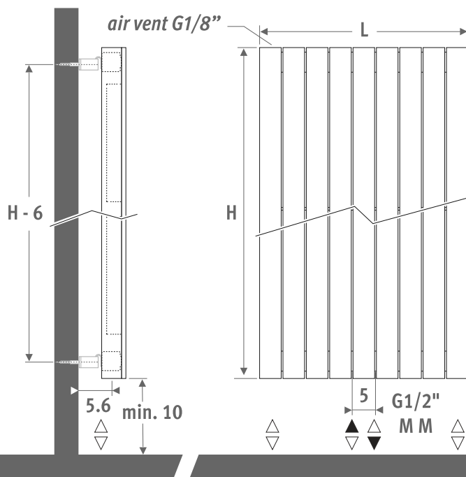
extended wall fixing
