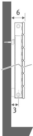
Type 11 standard wall fixing
