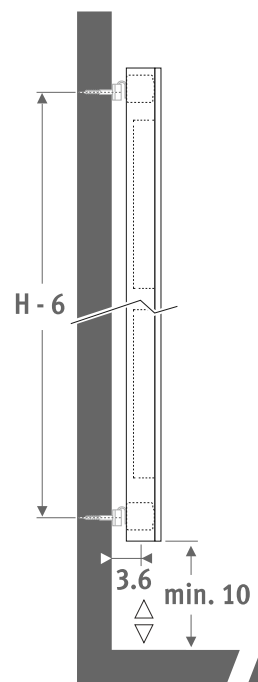
standard wall fixing
